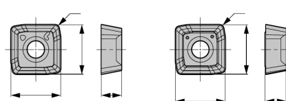
Fig. 3 Central insert L type Fig. 4 Central insert G type
